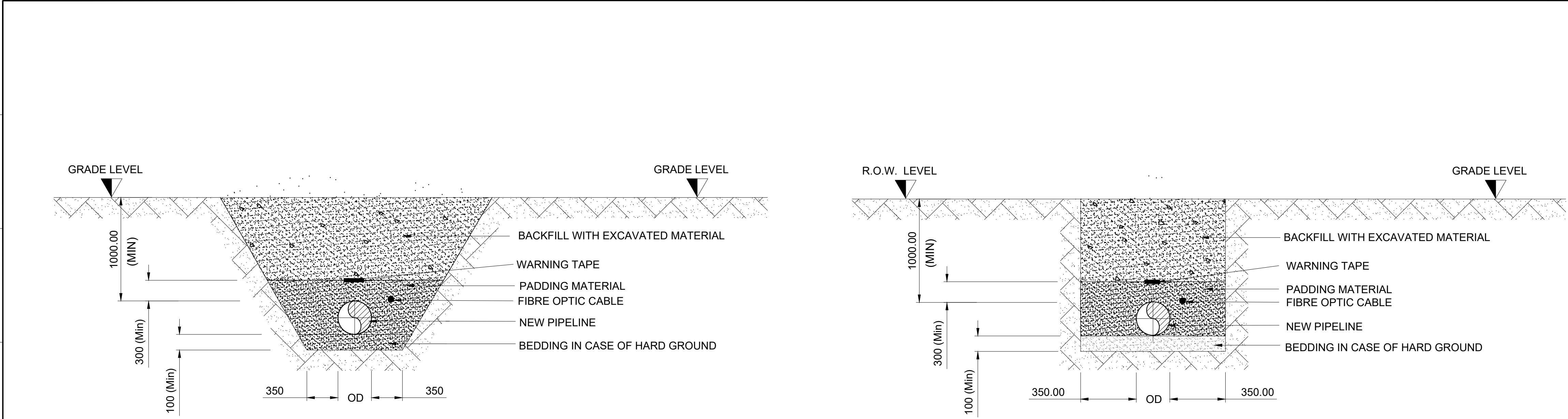
TRENCH IN ROCKY AREAS (IF ANY)
