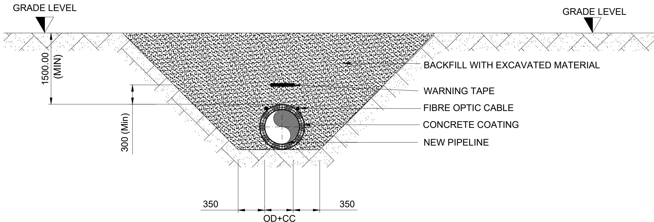
TRENCH IN SWAMP AREAS
